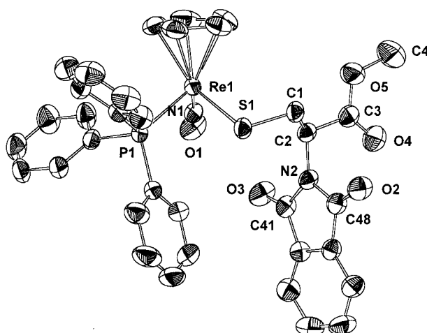
Figure 1. Molecular structure ( R,R )- [\text{CpRe}(\text{NO})(\text{PPh}_3)(\text{SCH}_2\text{CH}(\text{NC}_8\text{H}_4\text{O}_2)\text{COOMe})] ( 16a ) (without H atoms) [a]
